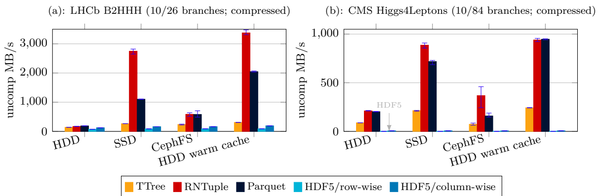
Figure 3. Read rate (uncompressed MB/s; 10 selected branches). Note the low ( < 10 MB/s) transfer rate for HDF5 in the CMS case.
