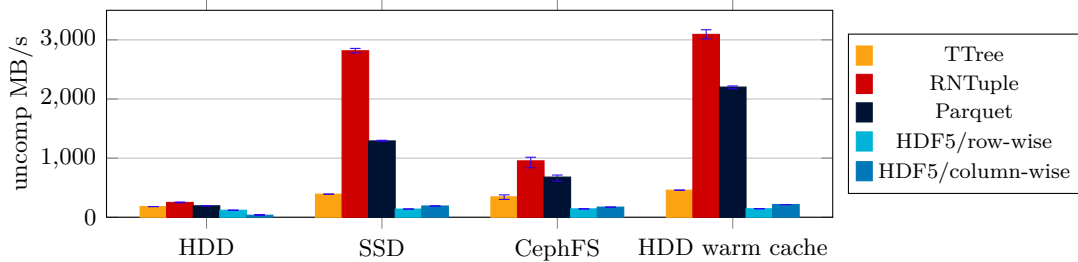
Figure 2. LHCb B2HHH analysis throughput (18/26 branches; compressed).
