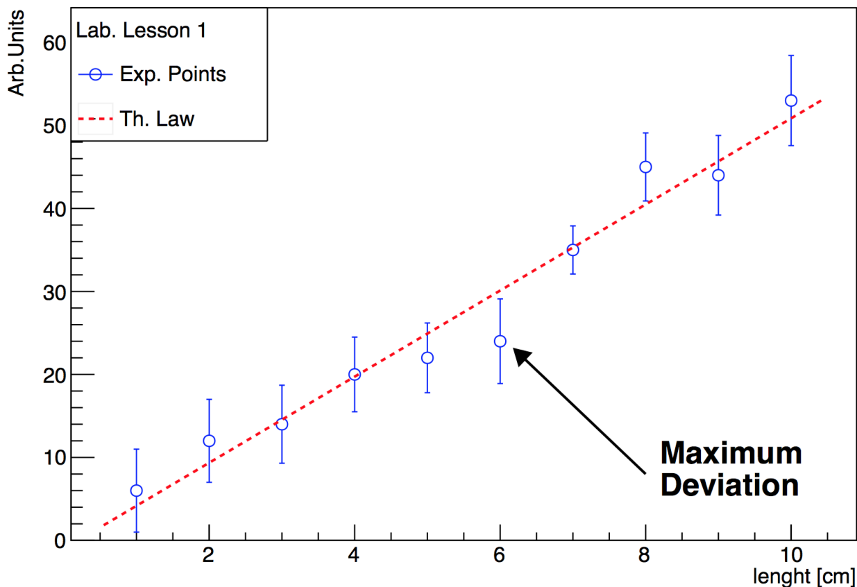
Figure 3.1: Your first plot with data points, a fit of an analytical function, a legend and some additional information in the form of graphics primitives and text. A well formatted plot, clear for the reader is crucial to communicate the relevance of your results to the reader.
