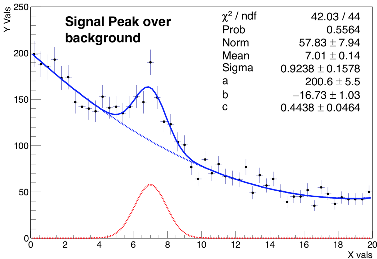
Figure 6.1: Fit of pseudo data: a signal shape over a background trend. This plot is another example of how making a plot “self-explanatory” can help you better displaying your results.
